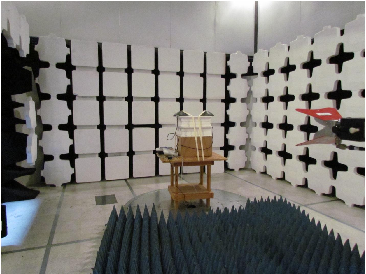
RDWN39 12 dBi RW-9401-5002 TX Spur 1-18G Front
