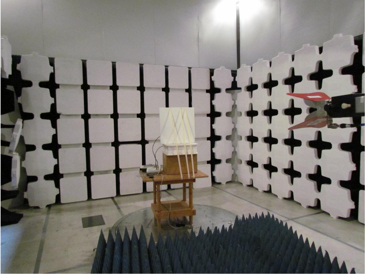
RDWN39 29 dBi Panel RW-9622-5001 TX Spur 1-18G Front
