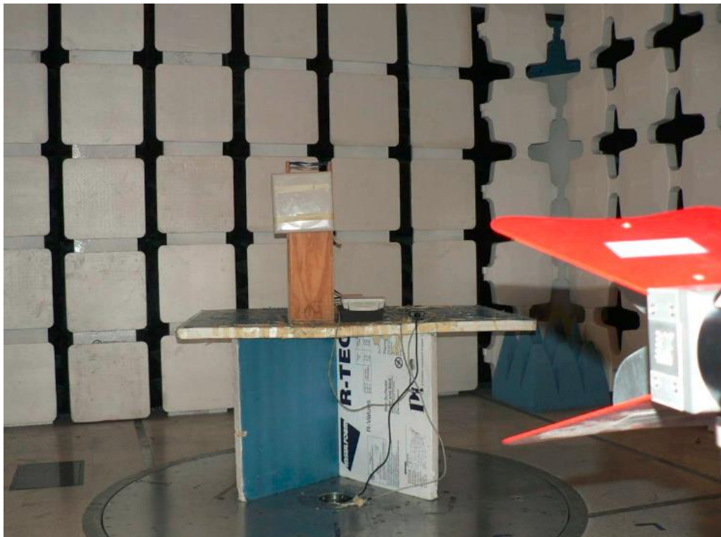
RDWN34 11 dBi MT0128930 TX Spur 1-18G Front
