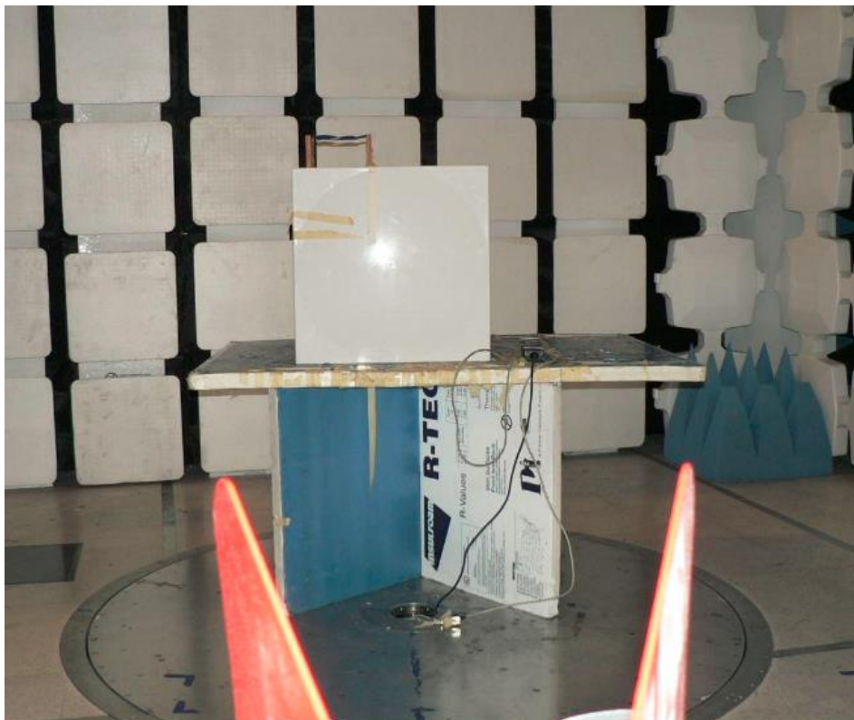
RDWN34 29 dBi Panel RW-9622-5001 TX Spur 1-18G Front
