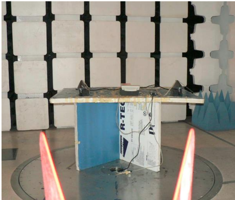
RDWN34 12 dBi RW-9401-5002 TX Spur 1-18G Front
