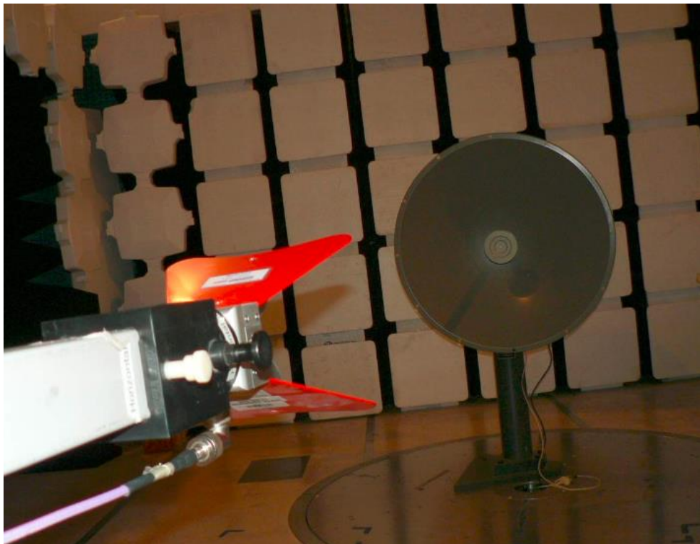
32 dBi Dish RW-9732-4958 TX Spur 1-18G Front
