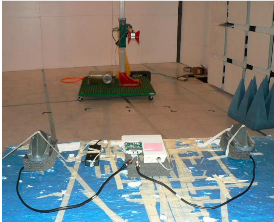
RDWN34 12 dBi RW-9401-5002 TX Spur 1-18G Front
