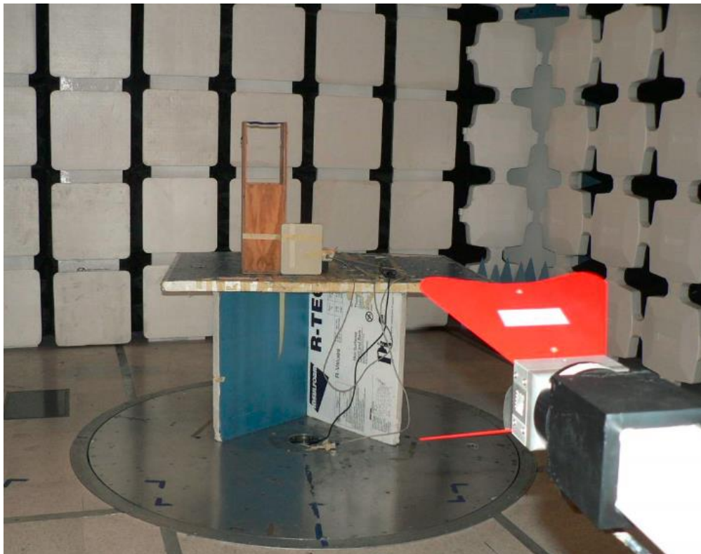
RDWN34 16 dBi ant AM0111760 TX Spur 1-18G Front
