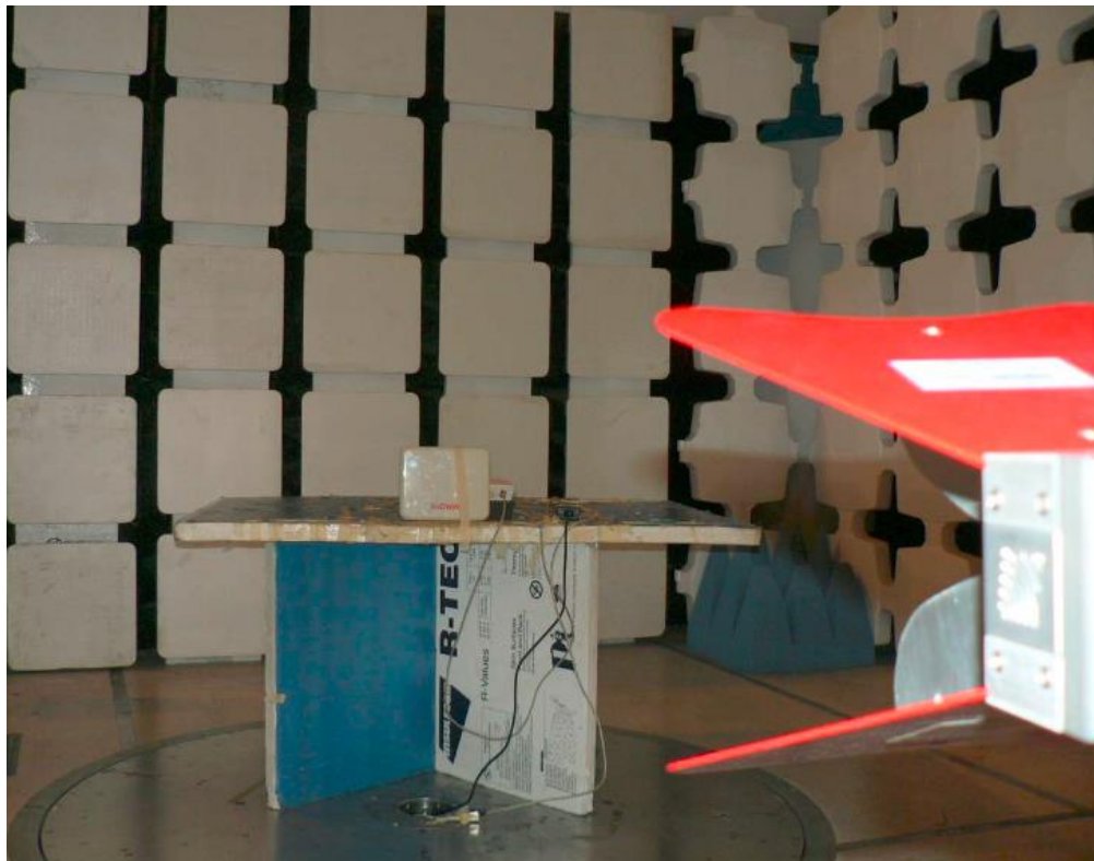
RDWN34 12 dBi AM0135060 TX Spur 1-18G Front
