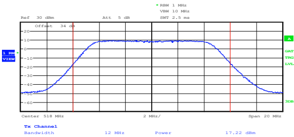
Figure 8.20-3: Attempt 1. Transmit conducted output power measurement. Limit 24 dBm
