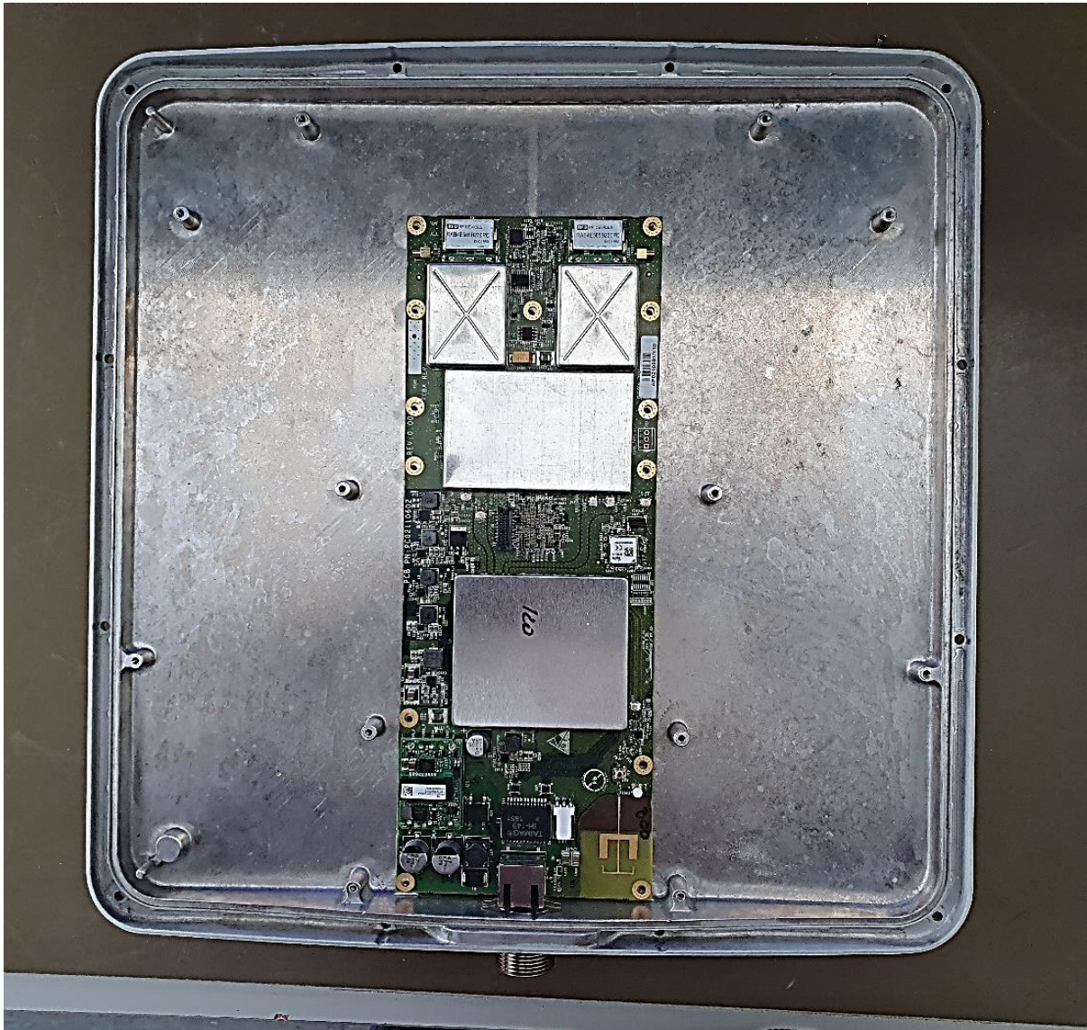
Photo 1: Internal Assembly View
