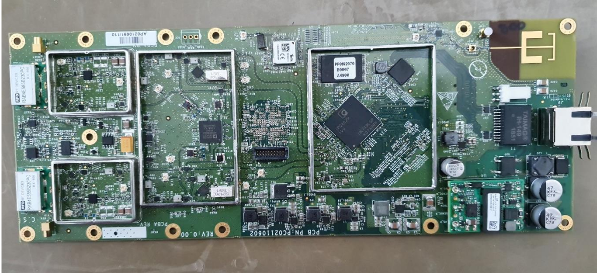
Photo 3: PCB C.S. view with shields off
