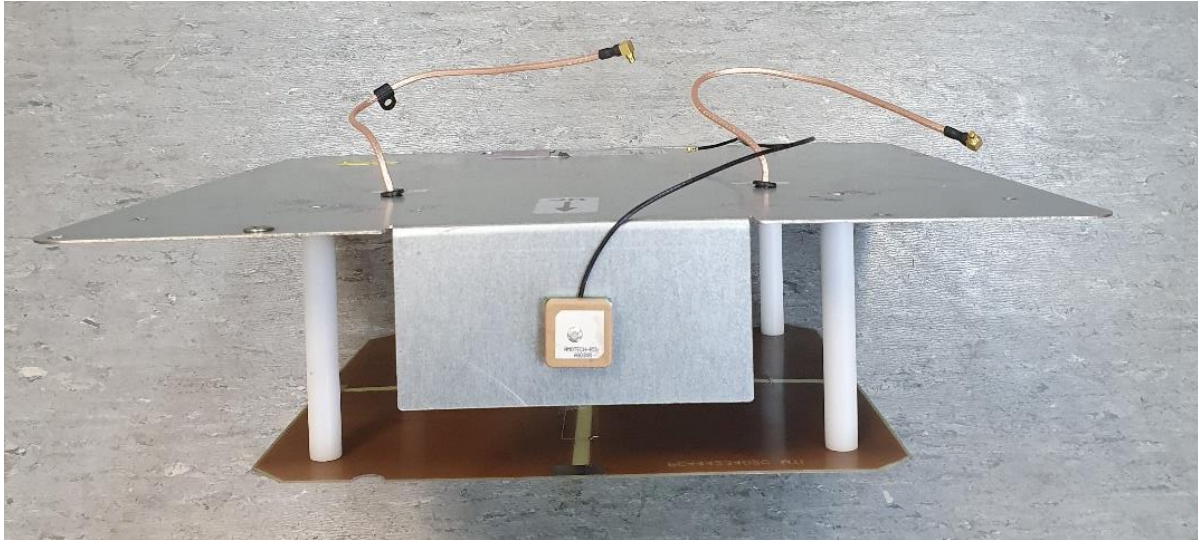
Photo 7: GPS module assembled on antenna
