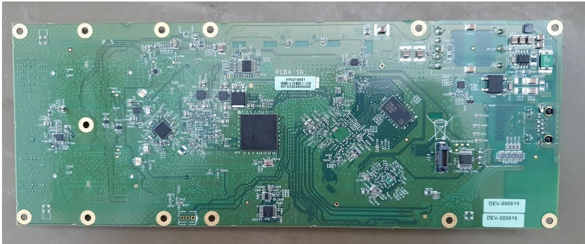
Photo 4: PCB P.S. view
