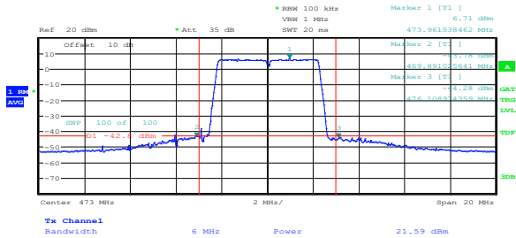
Figure 8.8-1: Conducted band edge and adjacent channel emissions sample plot for single 6 MHz channel
