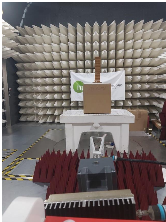
Figure 4. Radiated Emission Test, 18-26.5GHz
