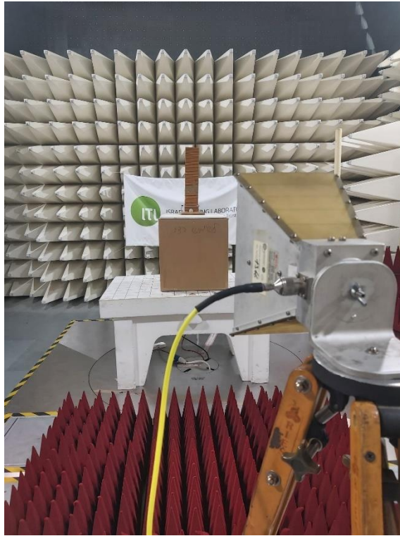
Figure 3. Radiated Emission Test, 1-18GHz
