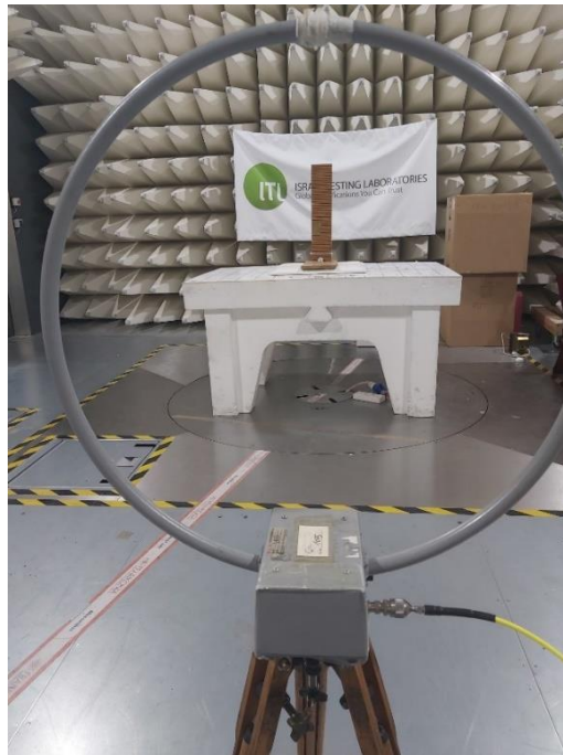
Figure 1. Radiated Emission Test, 0.009-30MHz
