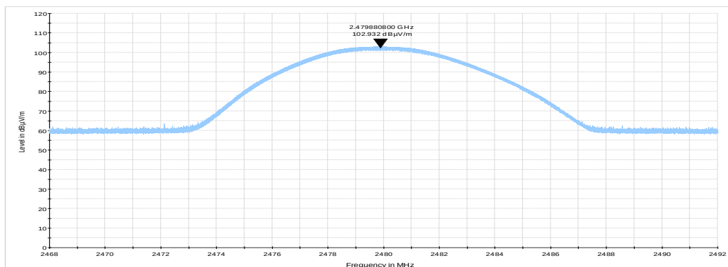
Plot 7.2.6 Field strength of carrier at high frequency with bitrate 2 Mbps
