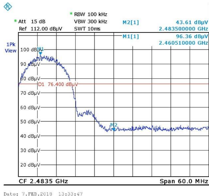
Figure 57 —Upper Band Edge, Wi-Fi/b 11Mbps
