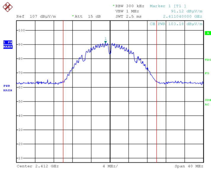
Figure 71 2412.0 MHz, Wi-Fi/b 1Mbps, Vertical
