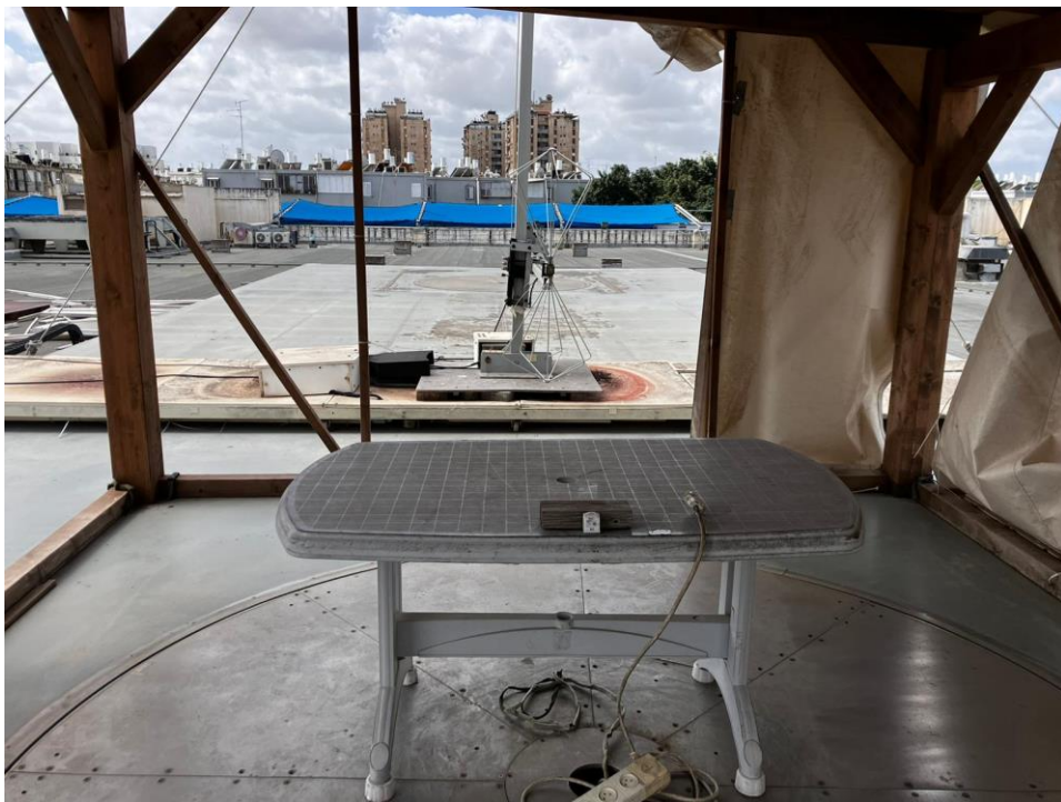
Figure 5. Radiated Emission Test, 30.0-200.0 MHz
