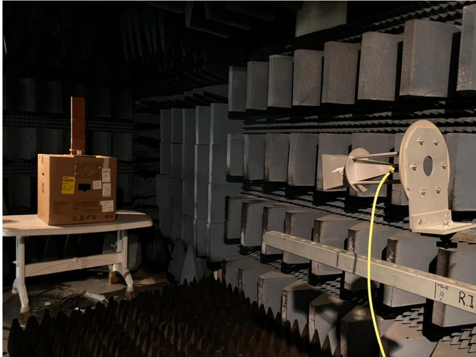
Figure 8. Radiated Emission Test, 18-26.5 GHz
