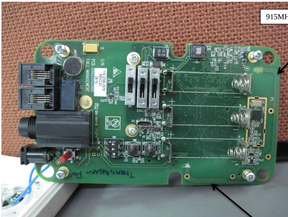
915MHz Side Antenna
