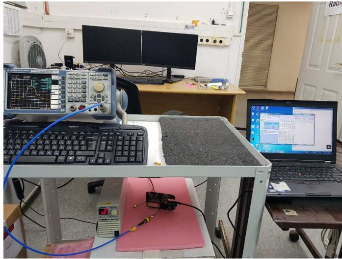
Figure 1. Conducted Emission Test (with Spectrum Analyzer)
