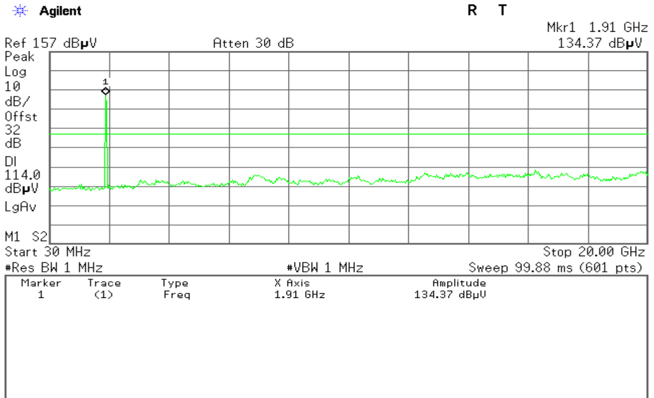
Figure 13-6: Out of Band emission at antenna terminals –EDGE CH High
