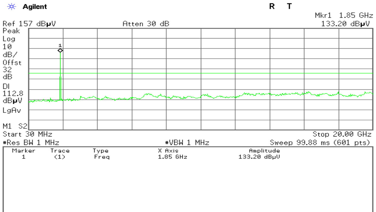
Figure 13-4: Out of Band emission at antenna terminals –EDGE CH Low
