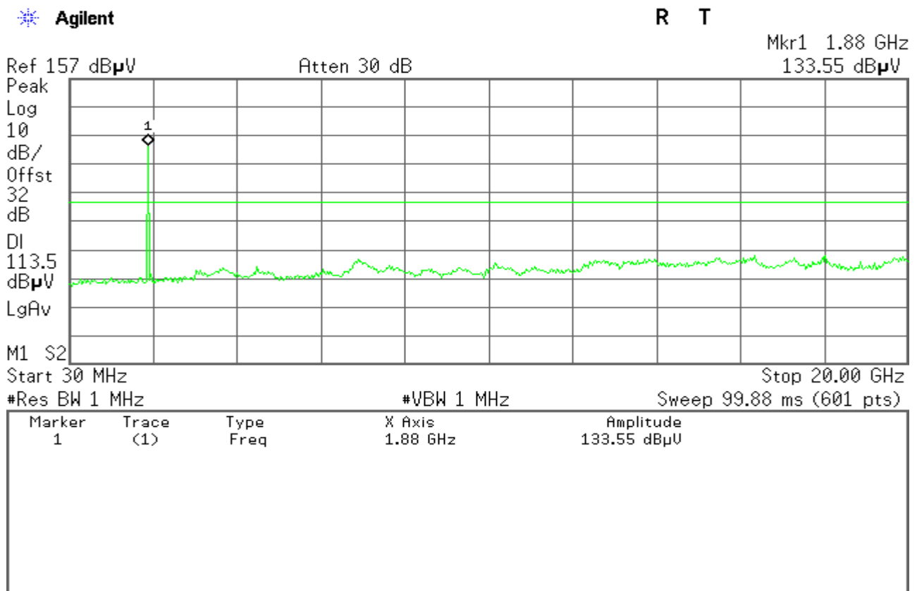
Figure 13-5: Out of Band emission at antenna terminals –EDGE CH Mid
