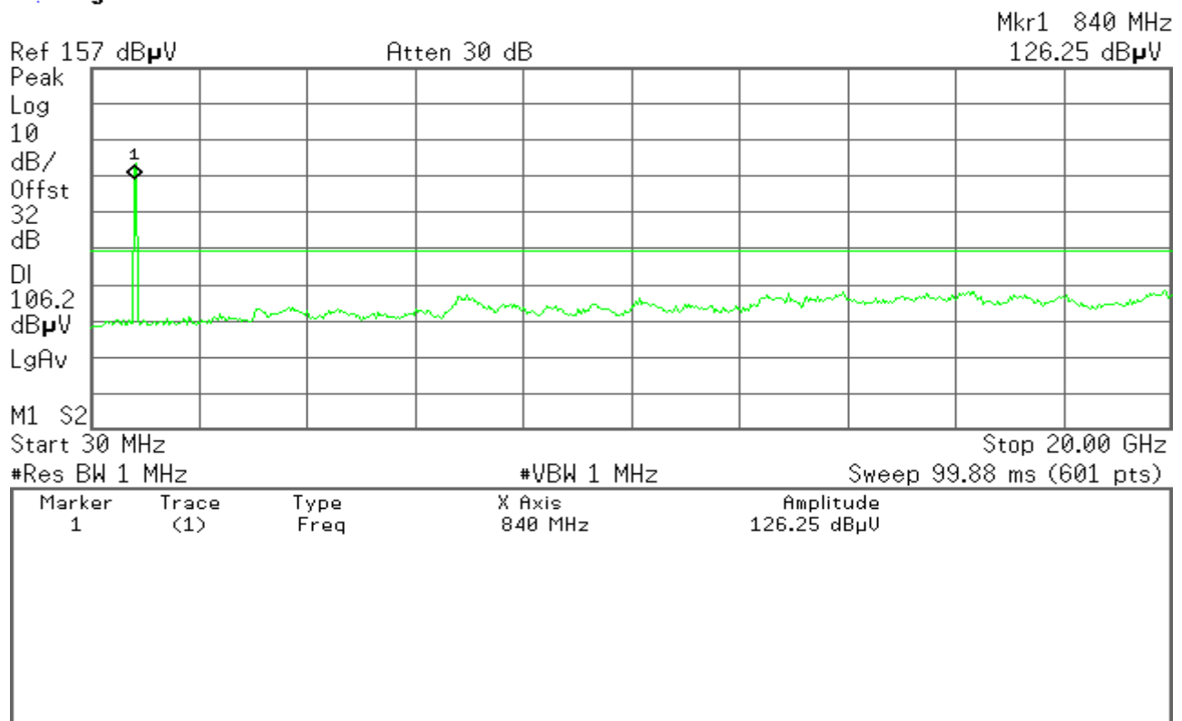
Figure 12-3: Out of Band emission at antenna terminals – HSUPA CH High
