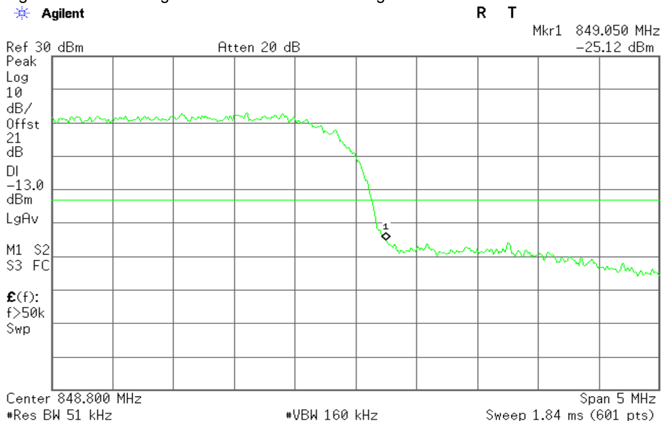
Figure 12-5: Band Edge emissions – HSUPA CH High
