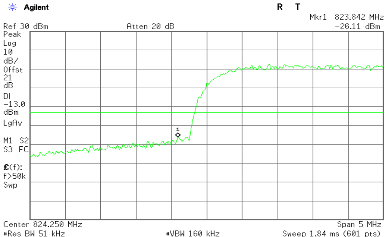
Figure 11-4: Band Edge emissions –WCDMA CH Low
