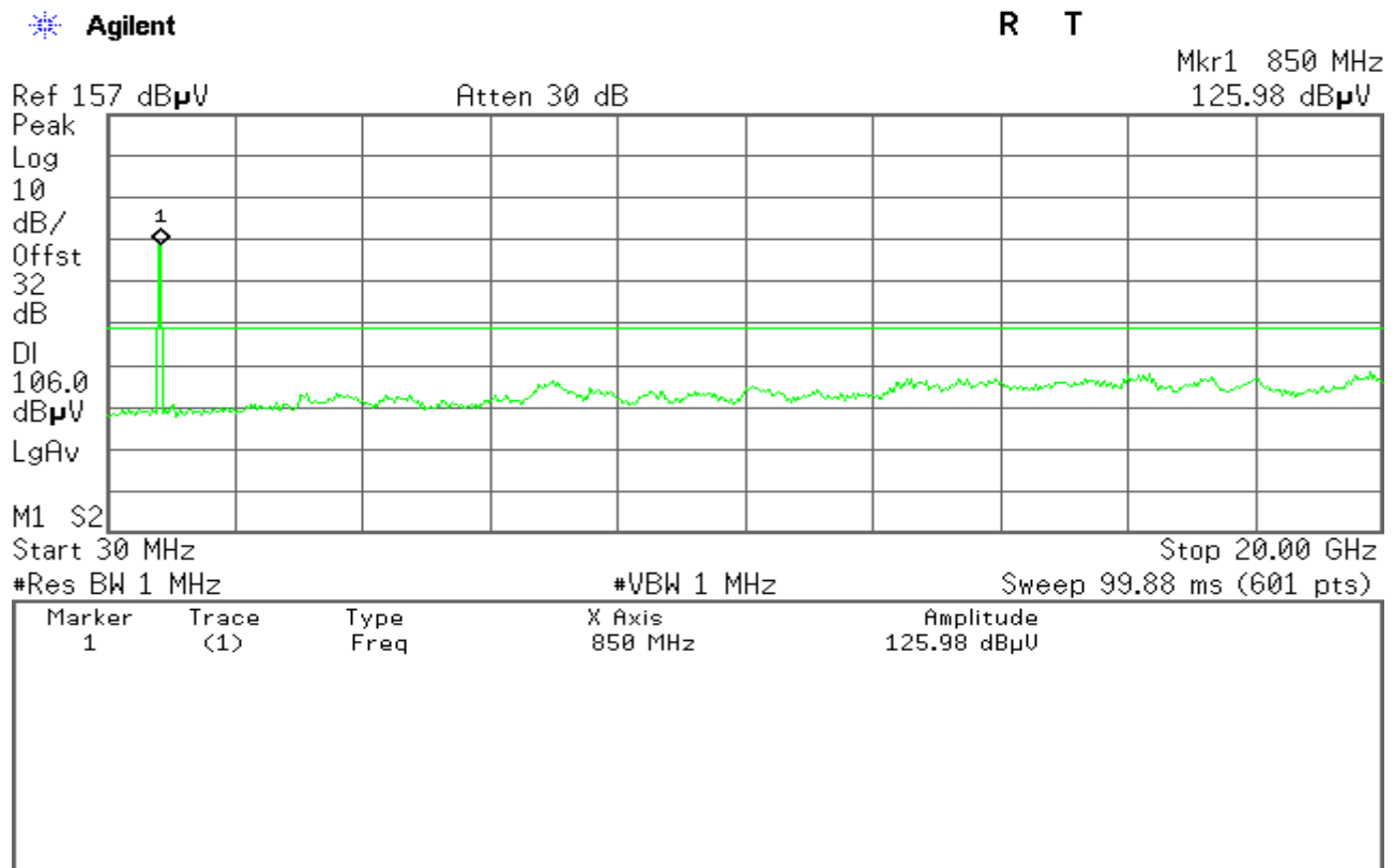
Figure 11-3: Out of Band emission at antenna terminals – WCDMA CH High
