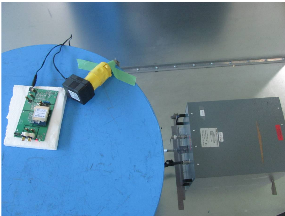
Figure 1: Power line conducted emission setup – photo 1
