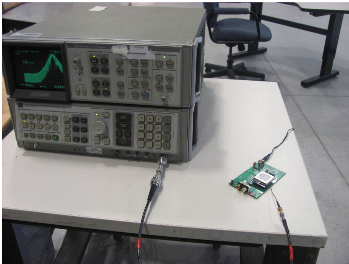
Figure 3: Antenna conducted emission setup – photo
