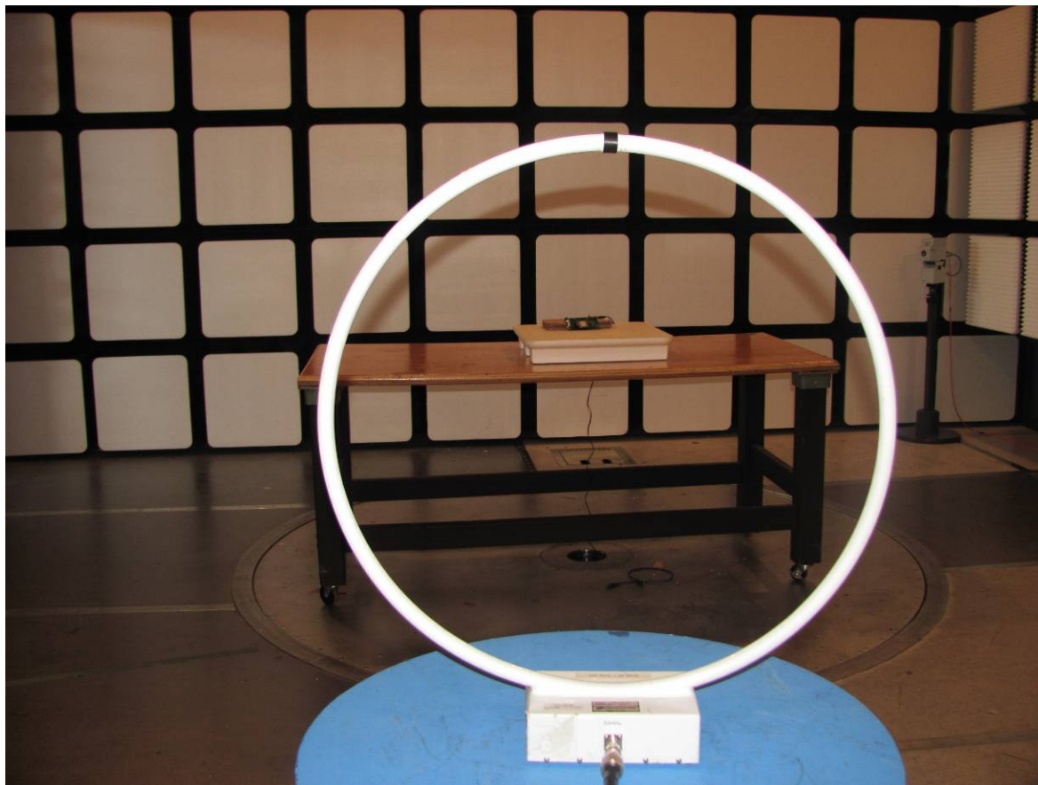
Figure 4: Radiated emission setup – photo 1
