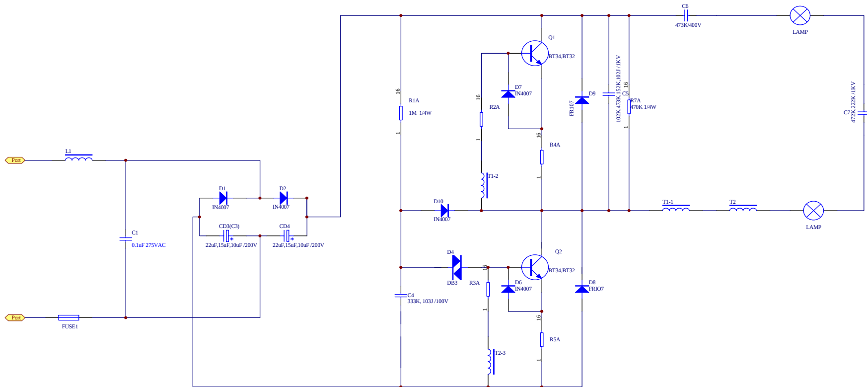
10W /15W/20W/25W CIRCUIT DIAGRAM
