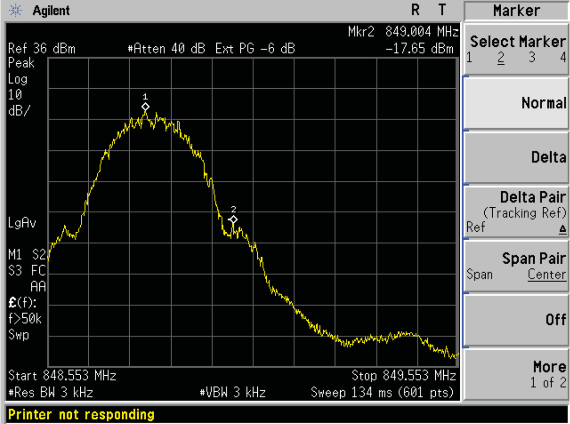
Higher Band Edge Plot on Channel 251
