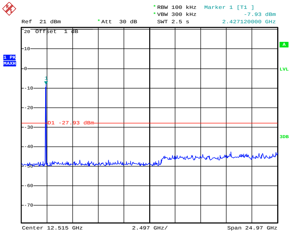
(Plot 4.6.4 A: Channel 3: 2422MHz @ 802.11n(40MHz))
