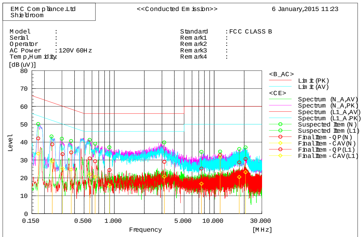
Figure 7. plot of Conducted Emission
