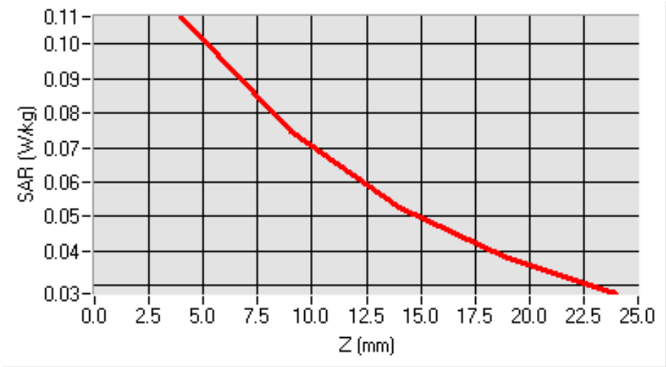
SAR, Z Axis Scan (X = 1, Y = -5)
