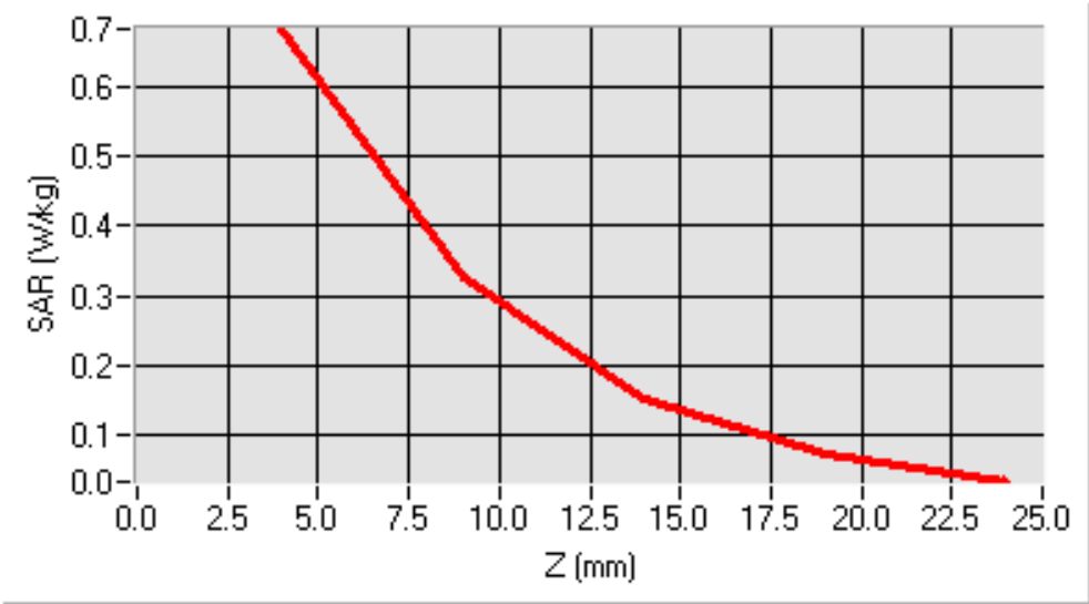
SAR, Z Axis Scan (X = -14, Y = 6)
