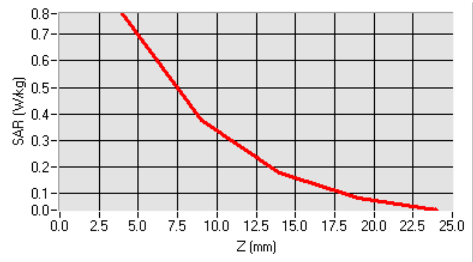
SAR, Z Axis Scan (X = -12, Y = -10)
