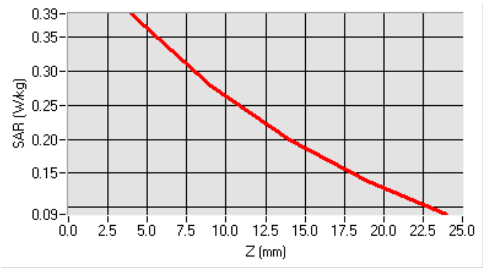
SAR, Z Axis Scan (X = -12, Y = 3)
