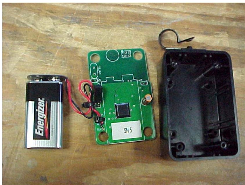
Inside the box and back view of the PCB
