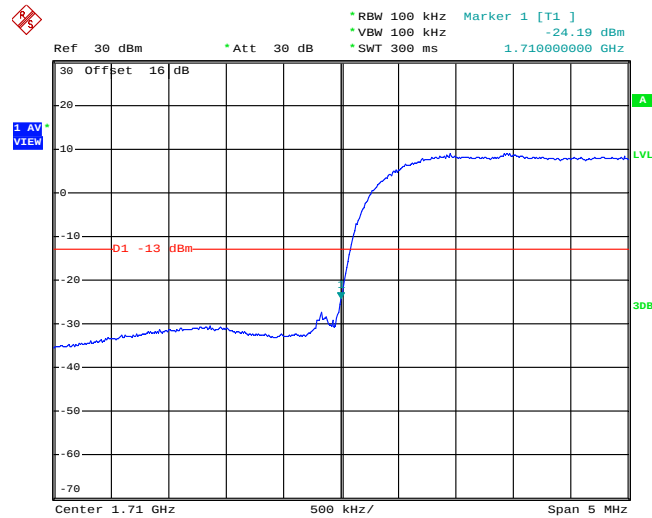
Lower Band Edge Plot on Channel 1312 (1712.4 MHz)
