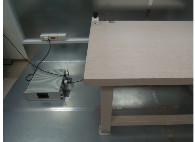
Conduction_Setup
