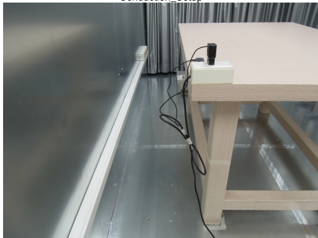
Conduction Setup
