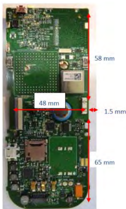
Fig.9 Antenna position of EUT (Back view)
