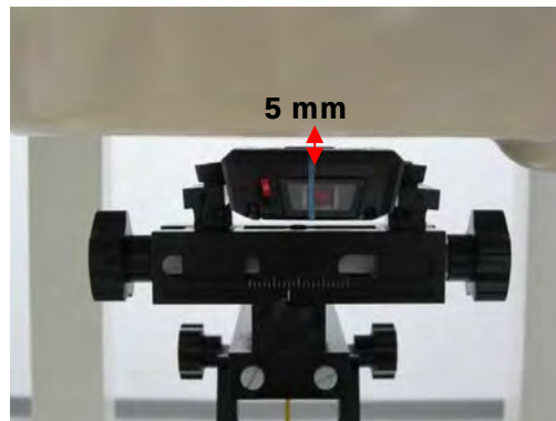
Fig.3 EUT front side to flat phantom
