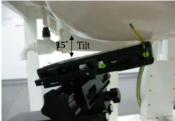
Fig.6 Left Head Section / Ear-Tilt Position(15°)
