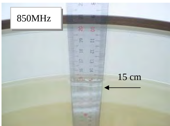
Fig.2.3 Flat (Body)
