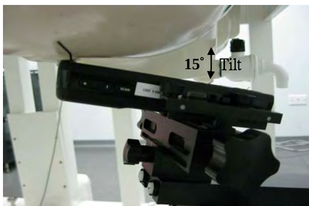
Fig.4 Right Head Section / Ear-Tilt Position(15°)
