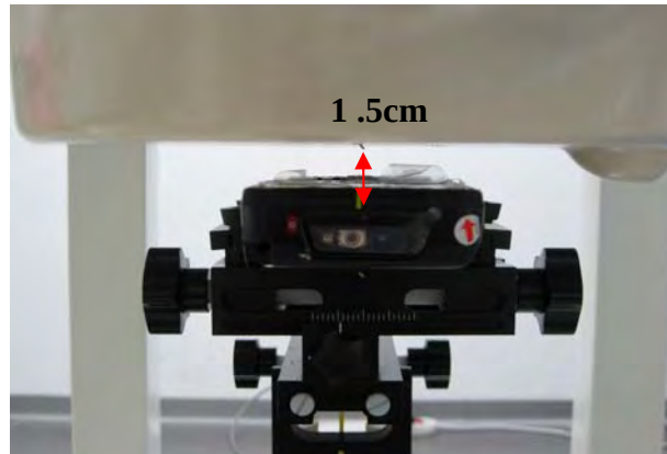
Fig.7 EUT front to flat phantom
