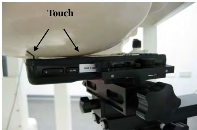
Fig.3 Right Head Section / Cheek-Touch Position
