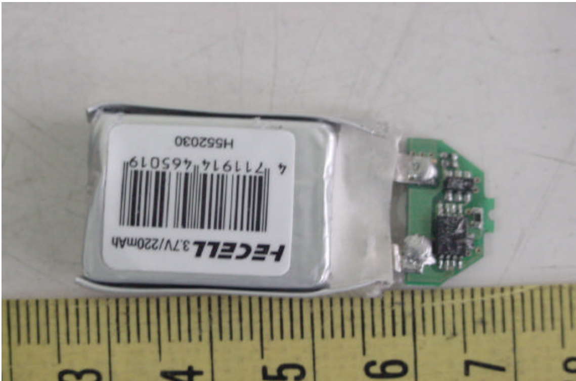
Internal View of Battery
