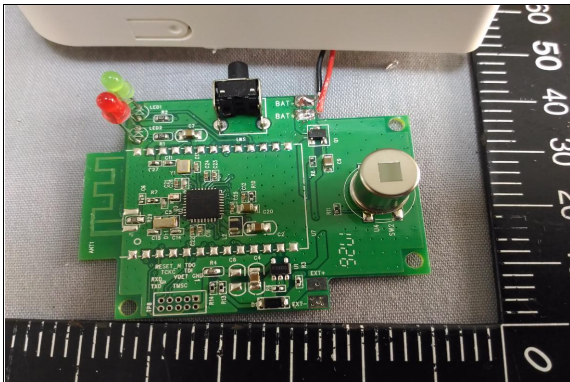
< PCB-F >
