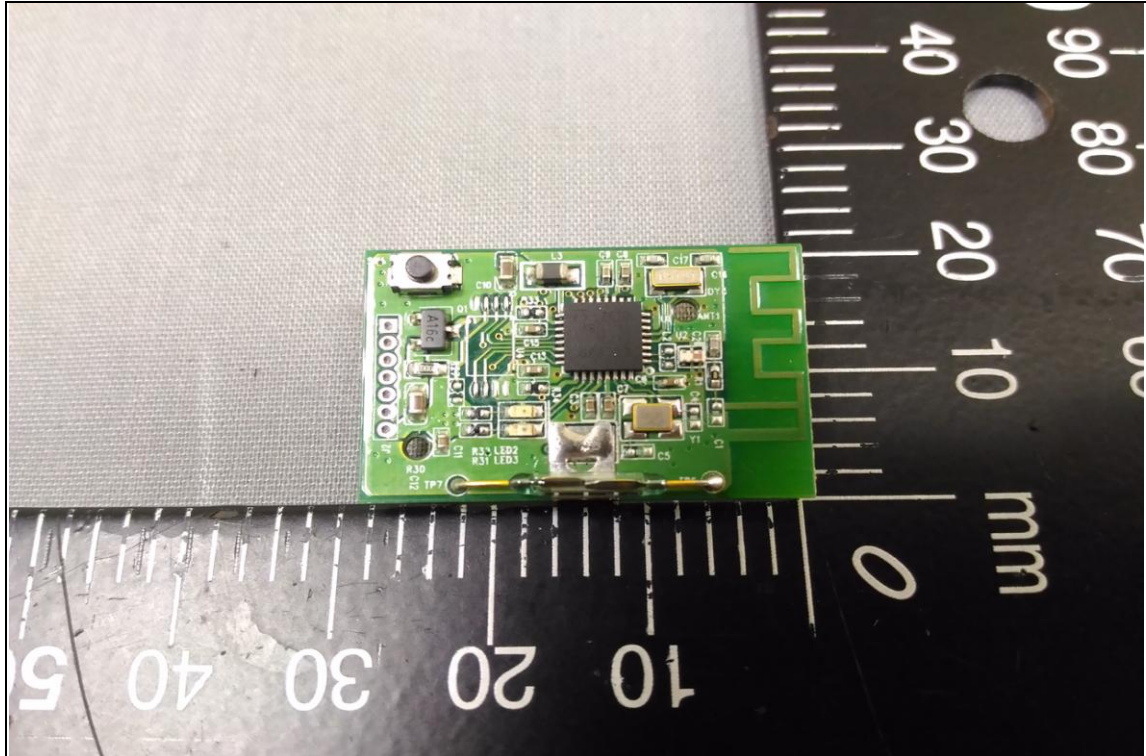
< PCB-R >
