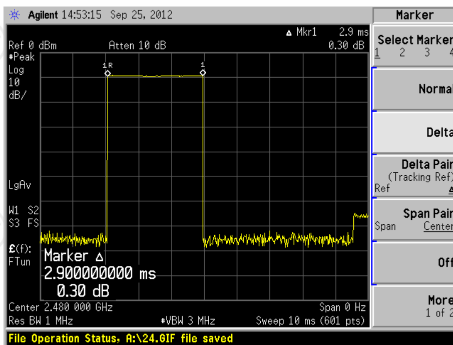
Channel 79_ 2480 MHz_DH5
