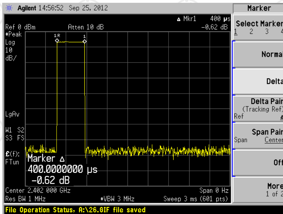
Channel 1_ 2402 MHz_DH1
