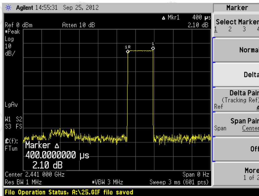
Channel 40_ 2441 MHz_DH1
