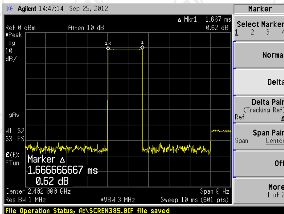
Channel 1_ 2402 MHz_DH3
