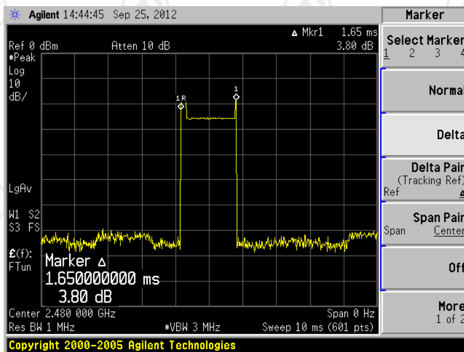
Channel 79_ 2480 MHz_DH3
