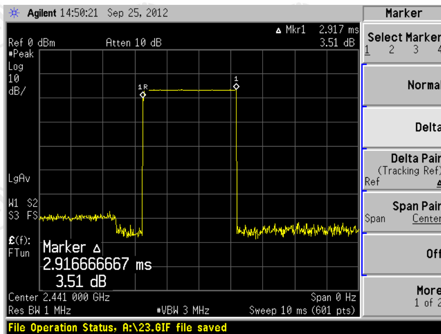
Channel 40_ 2441 MHz_DH5
