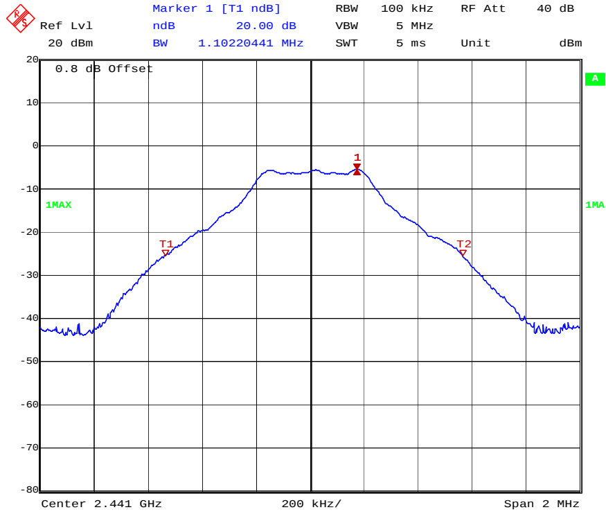
20dB Bandwidth (1Mbps)
