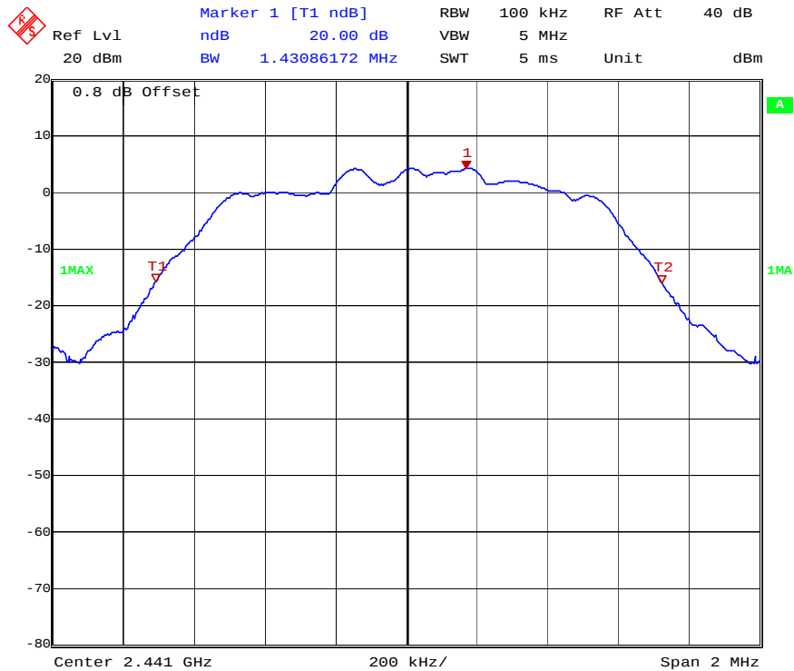
20dB Bandwidth (2Mbps)
