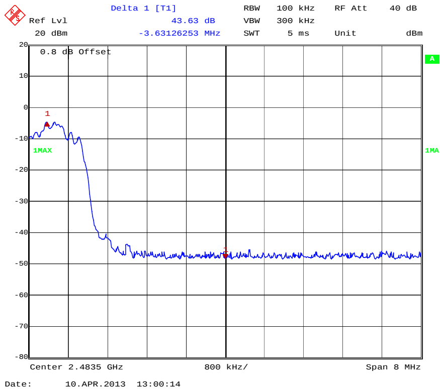
Conducted Band Edge High Channel (3Mbps)
