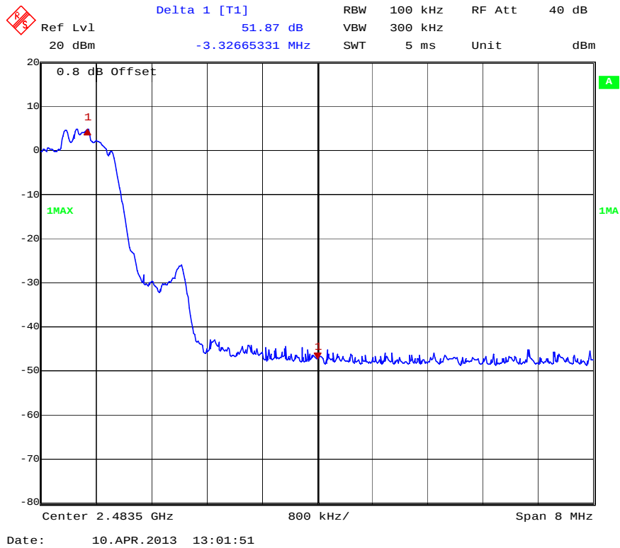
Conducted Band Edge High Channel (2Mbps)
