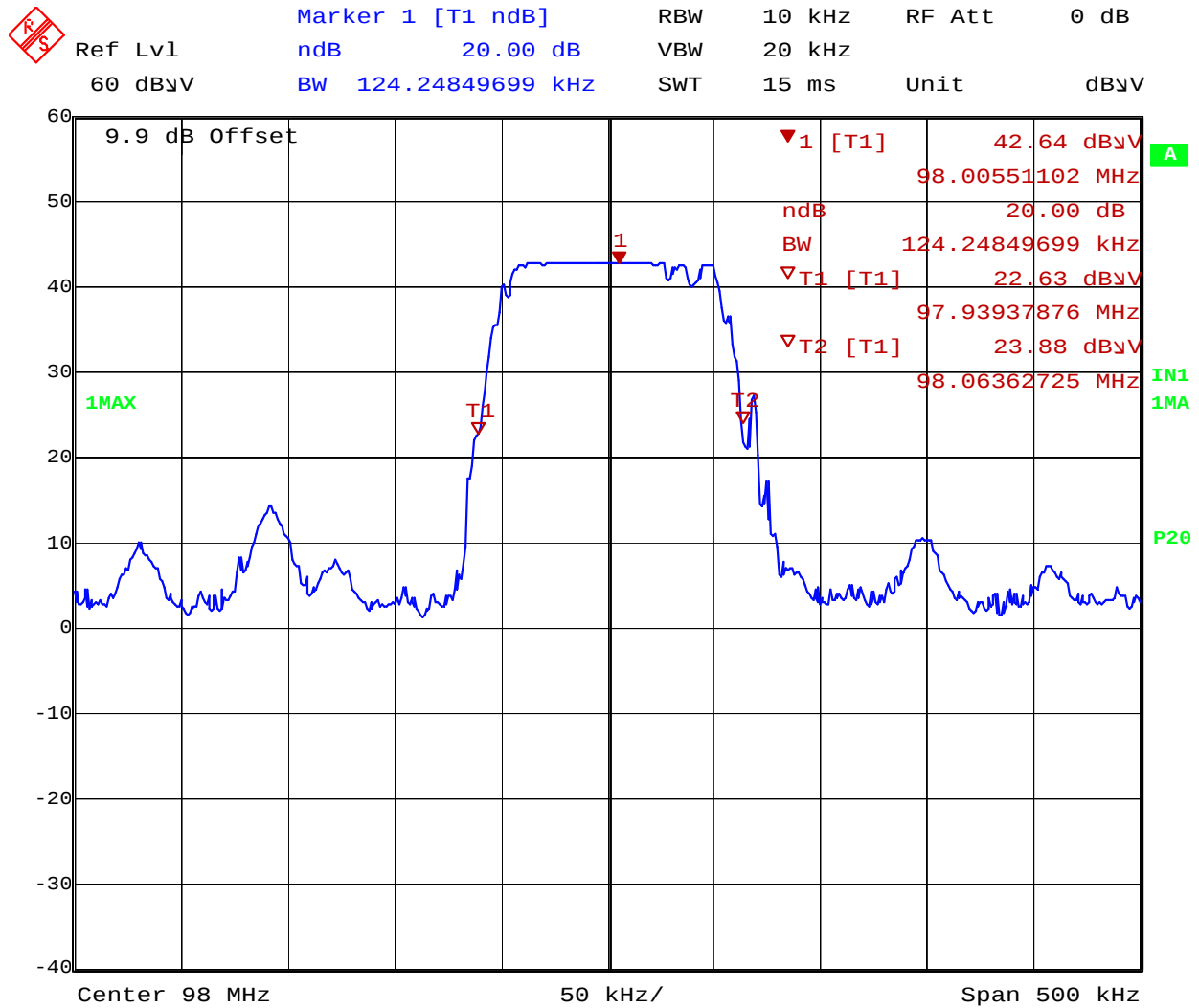
20dB Bandwidth Plot (98MHz)
