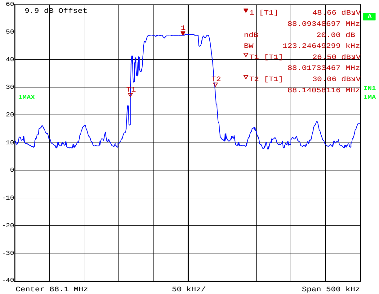
20dB Bandwidth Plot (88.1MHz)
