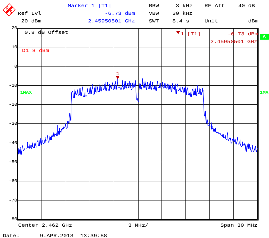
Power Spectral Density – Channel 11 802.11g mode
