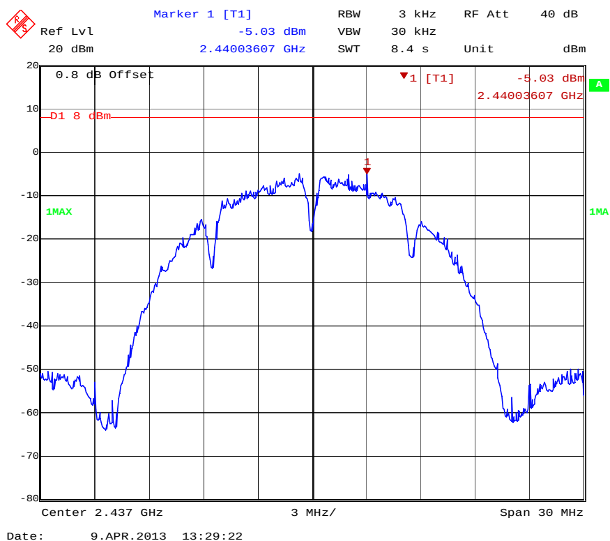
Power Spectral Density – Channel 6 802.11b mode
