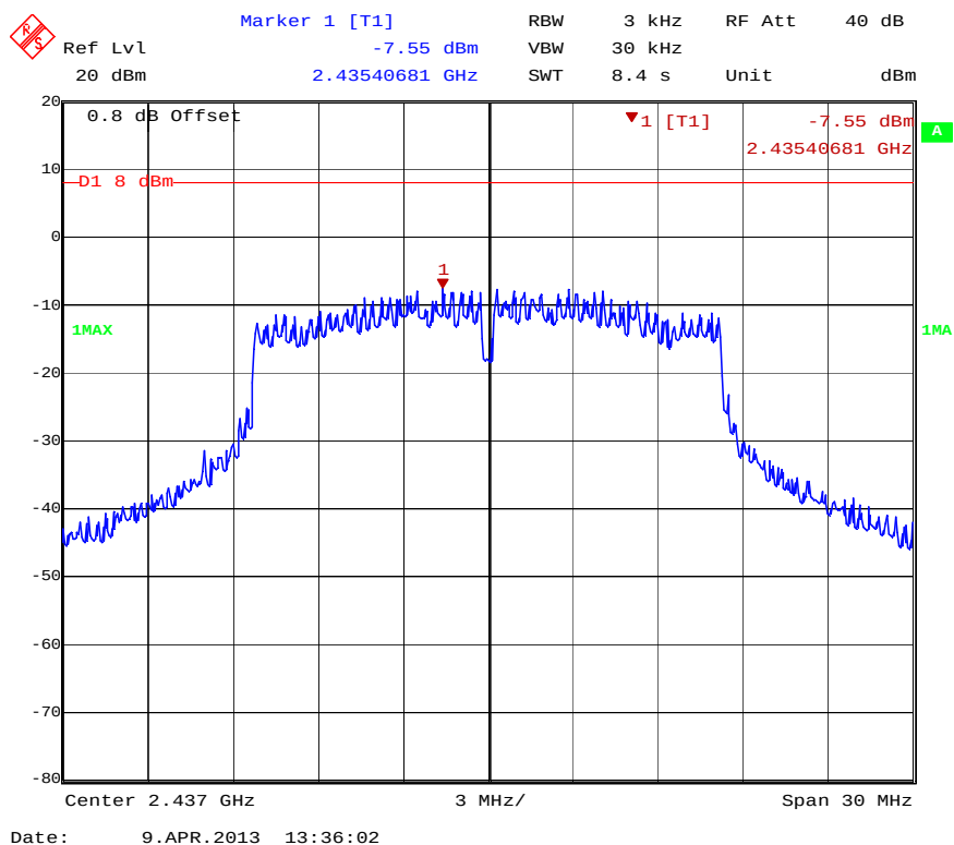
Power Spectral Density – Channel 6 802.11g mode
