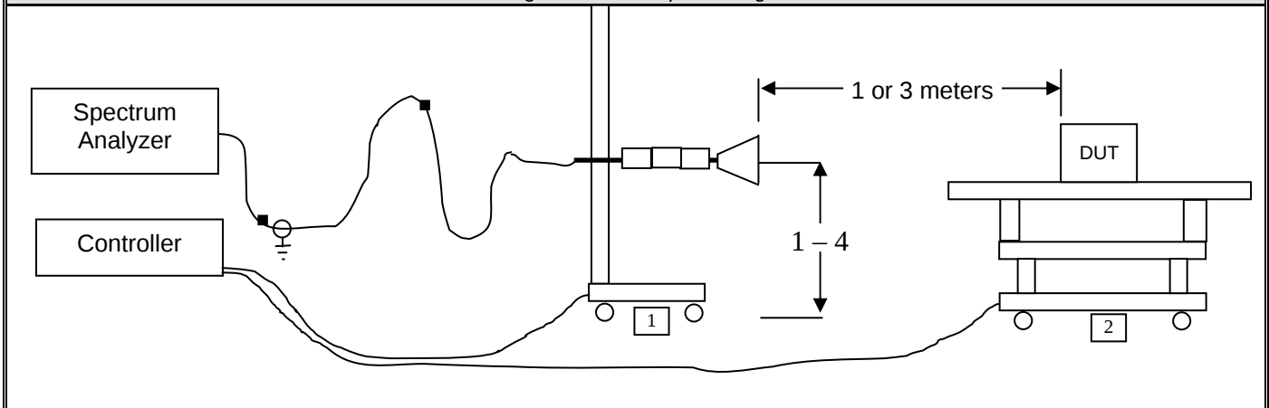
Figure 7-1 - Setup Drawing
