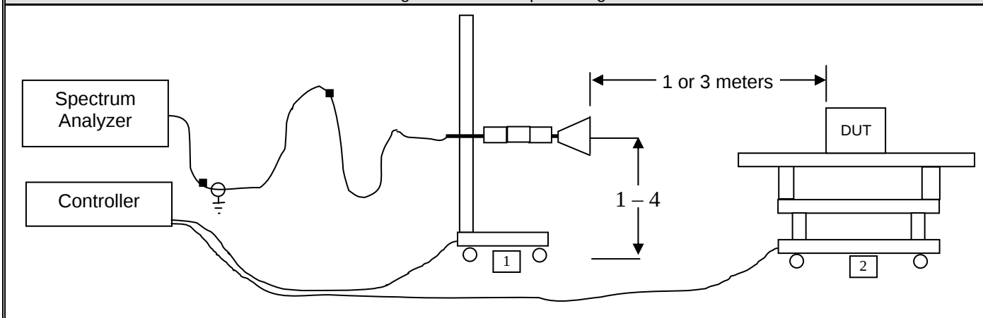
Figure B.7-1 - Setup Drawing
