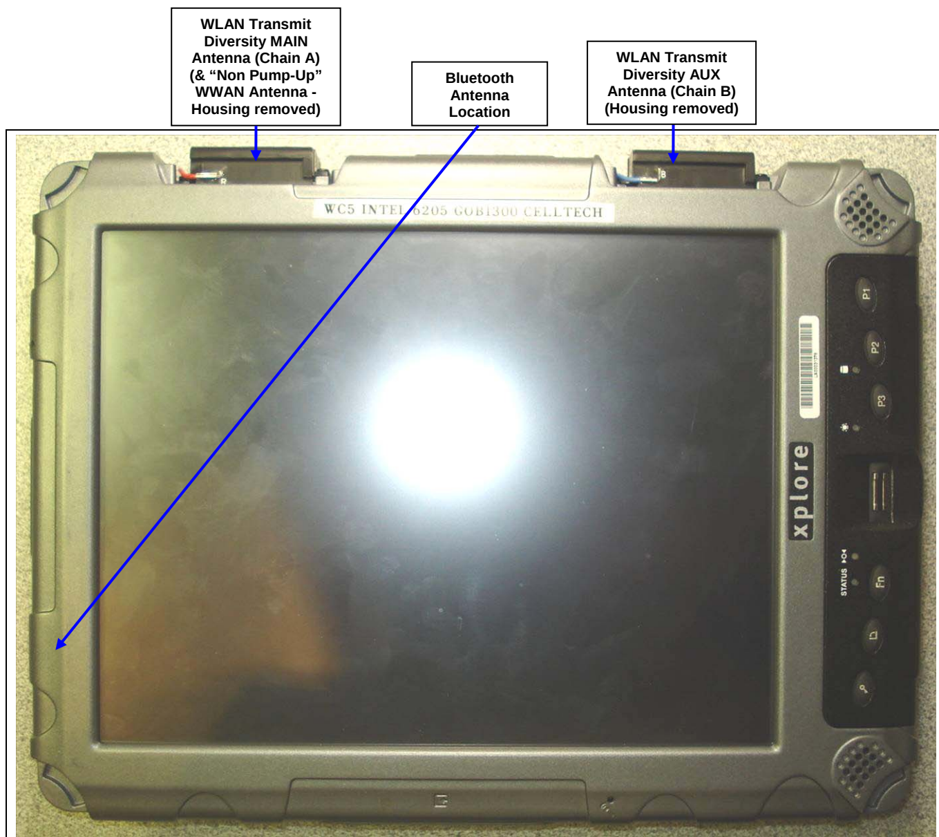
WLAN & BLUETOOTH ANTENNA LOCATIONS - TOP SIDE OF iX104C5 TABLET PC
