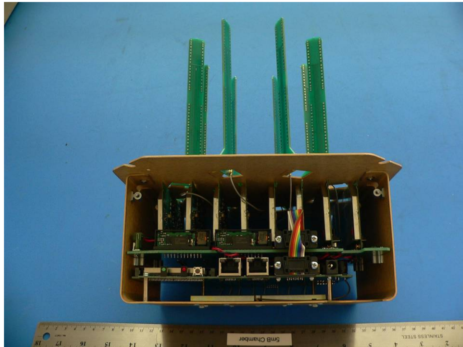
EUT - Chassis off Rear connector View 2
