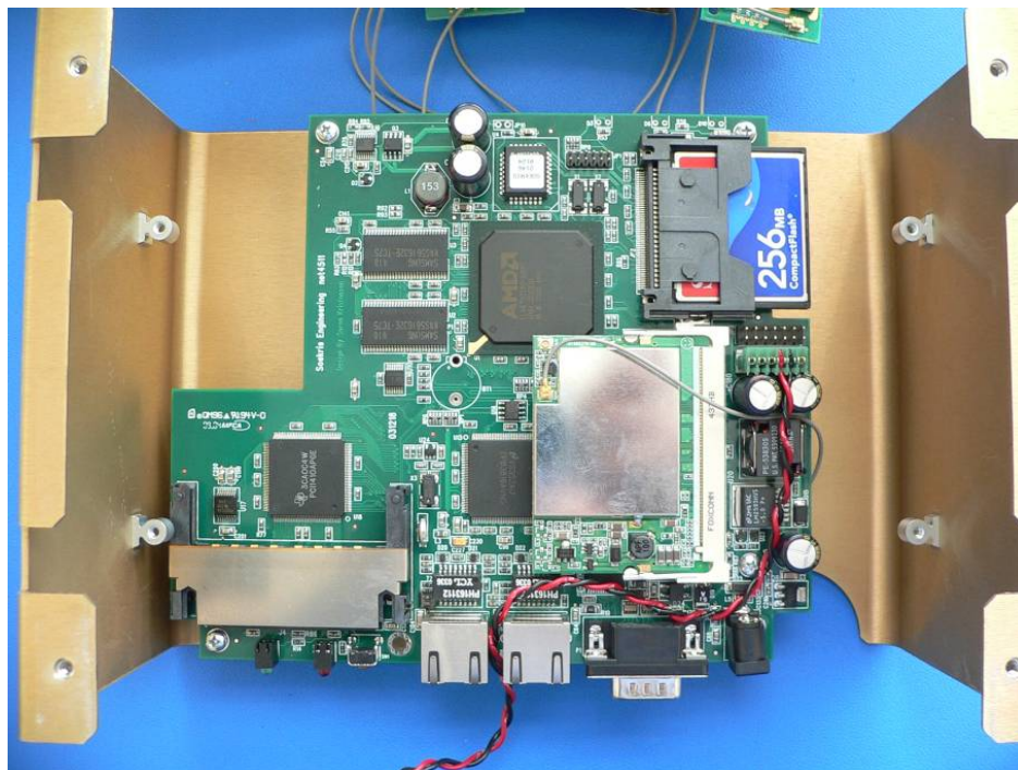
EUT - Antenna off Top view 1
