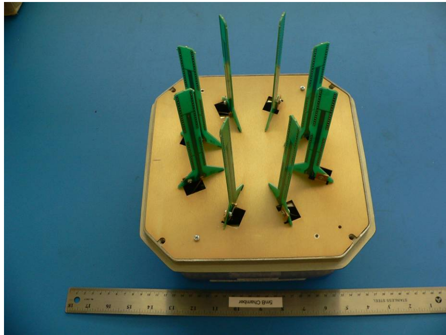
EUT - Chassis off front View 2
