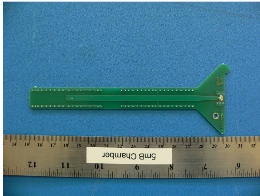
EUT - Antenna PCB Component Side View
