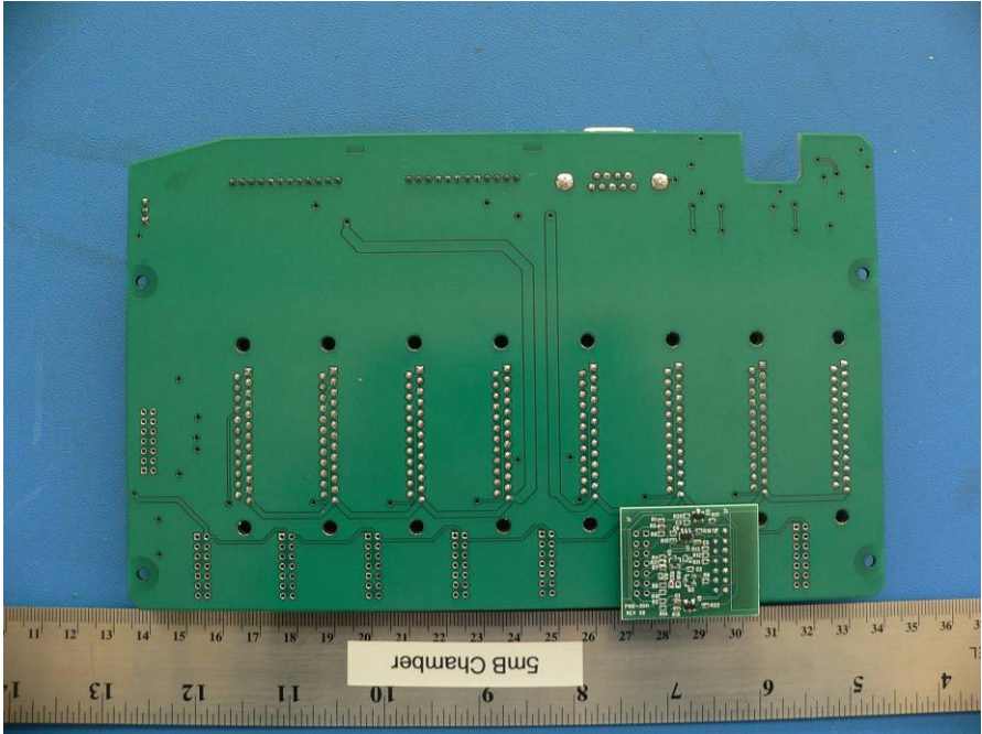
EUT - Sub PCB Solder View 1
