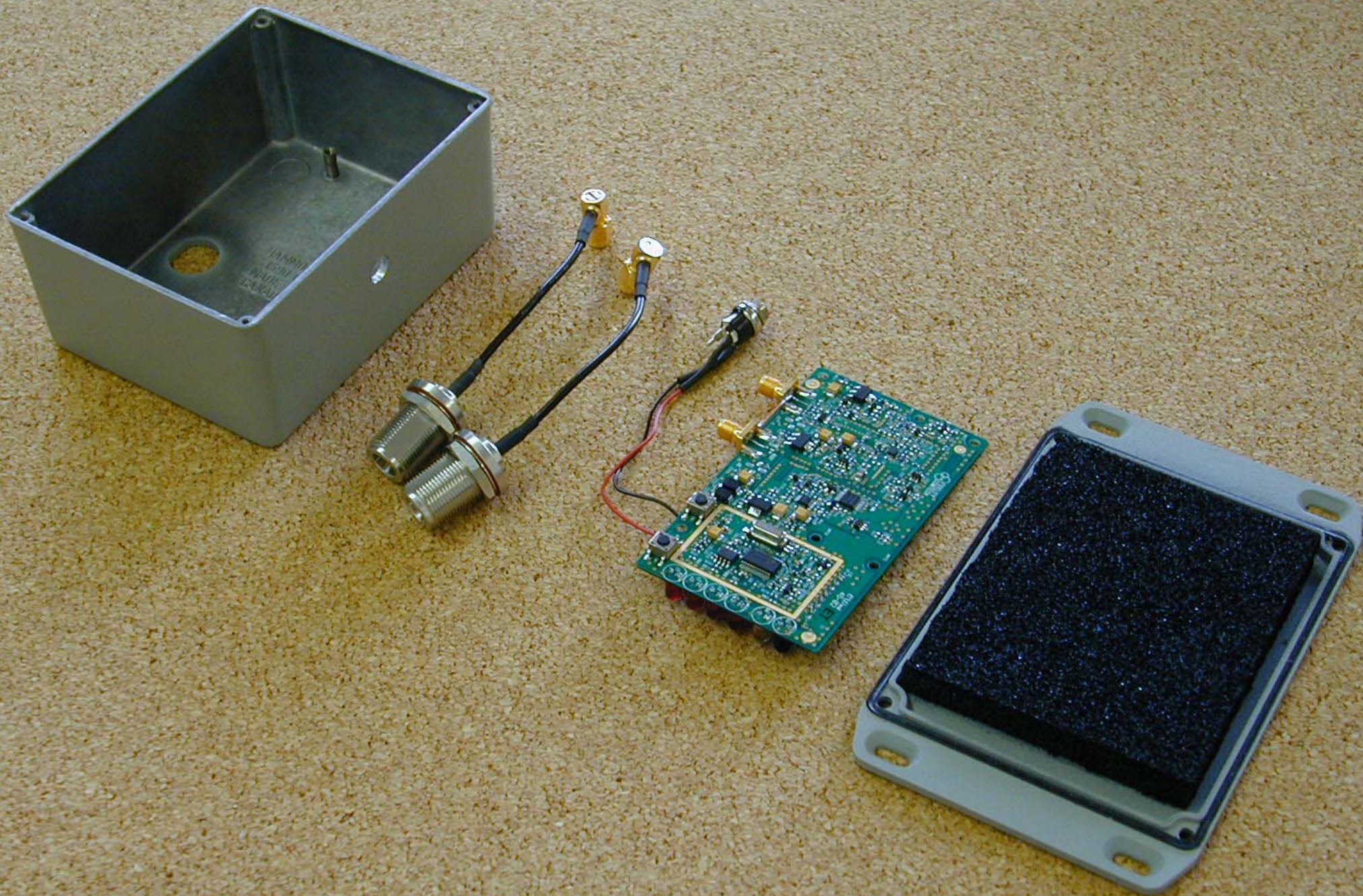
FCI-2401i Indoor Power Amplifier - Apart (Bottom)
