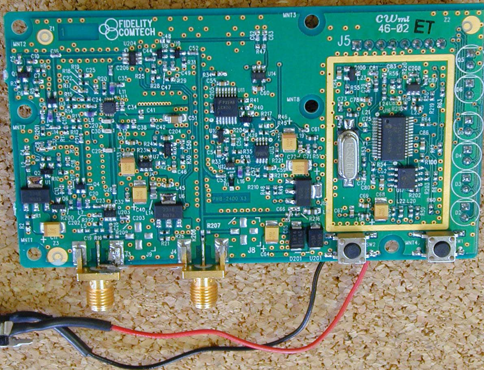
FCI-2401i Indoor Power Amplifier PCB (Top)
