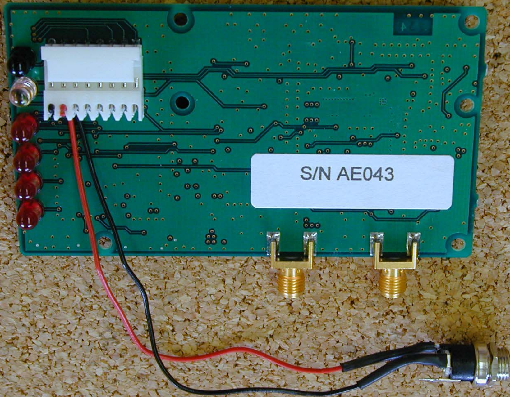
FCI-2401i Indoor Power Amplifier PCB (Bottom)
