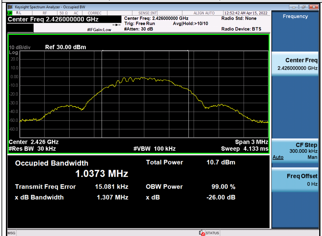
Test_Graph_LE1M_ANT1_2426_1Mbps_OBW
