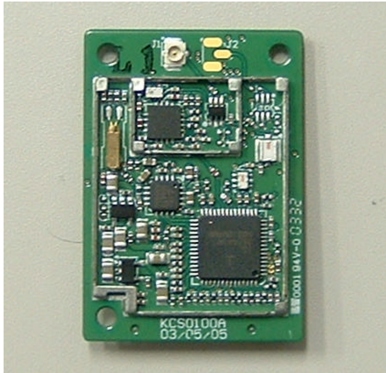
Module Front (without Shield)
