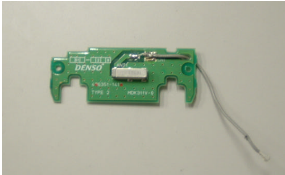
Antenna Front
