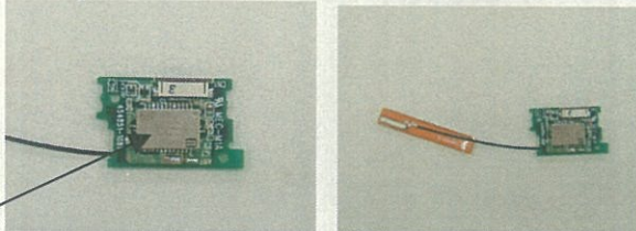
A1 Photo(Modular transmitter)
