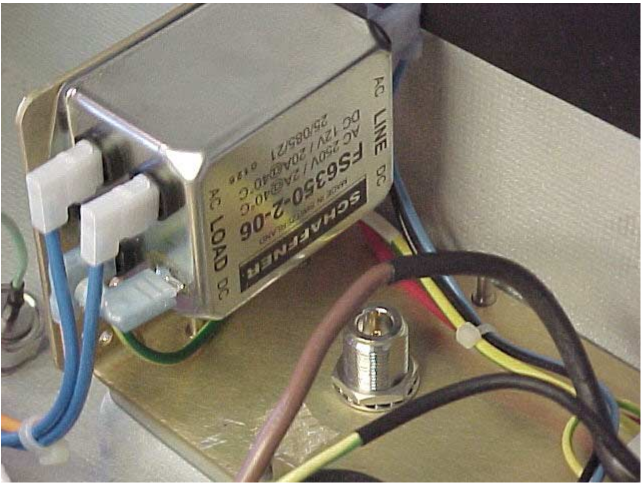
AC_DC Filter
