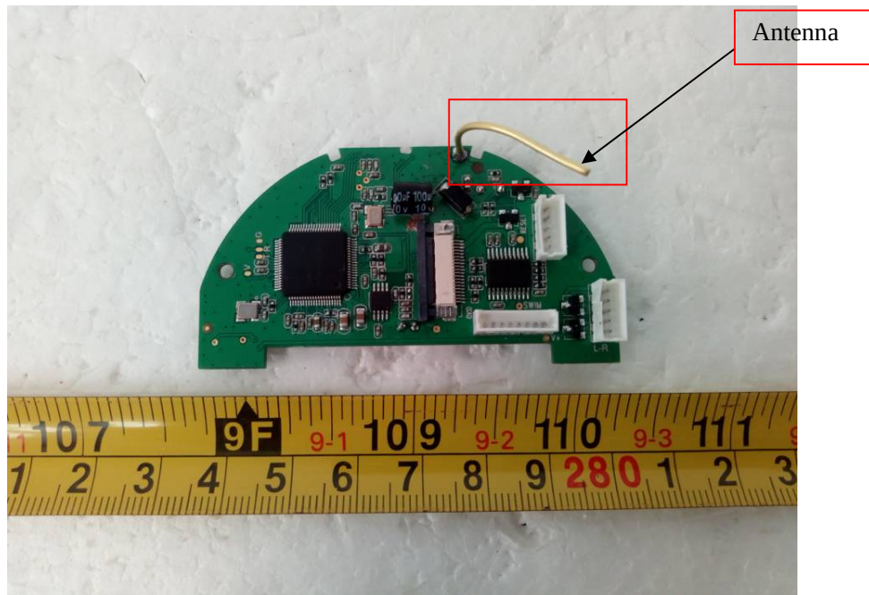
EUT – Main Board 1 Top View
