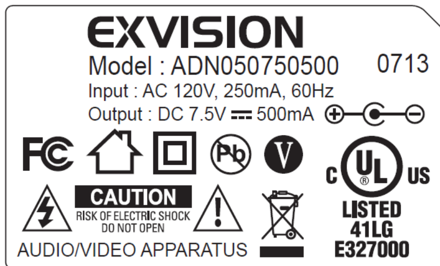
EUT – Adapter Label View
