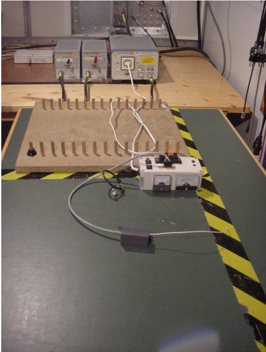
Photo 5 (Conducted Emissions):
