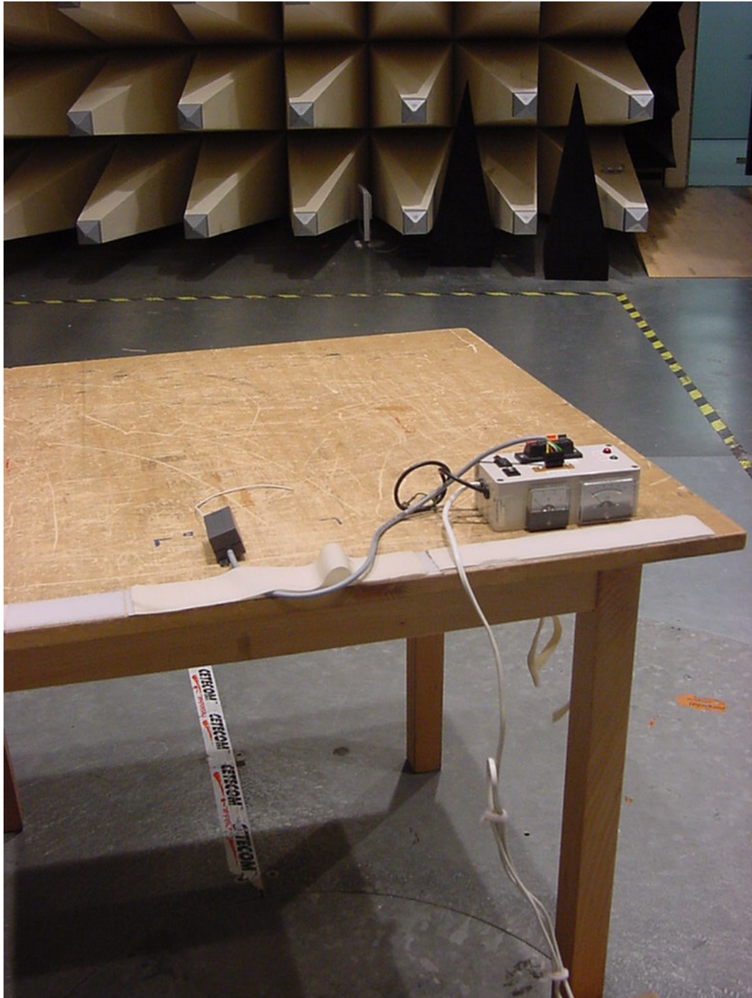
Photo 4 (Radiated Emissions):HE2-315
