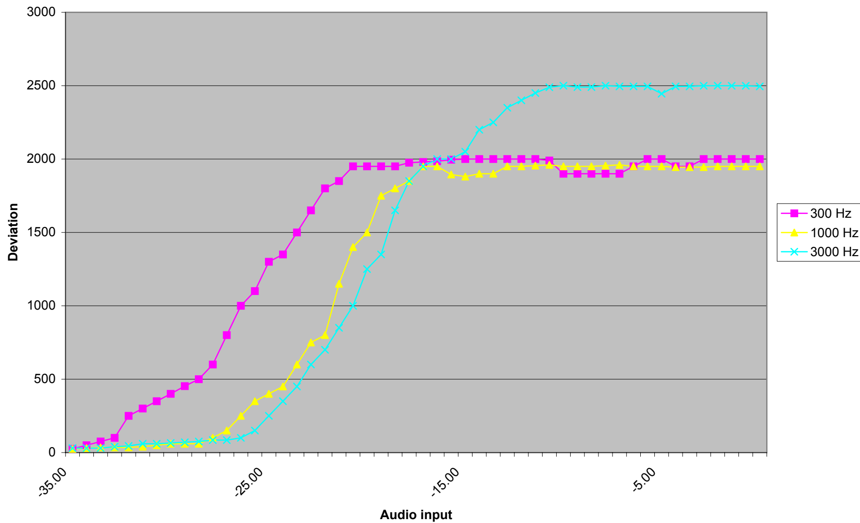
Modulation Limiting 12.5 kHz
