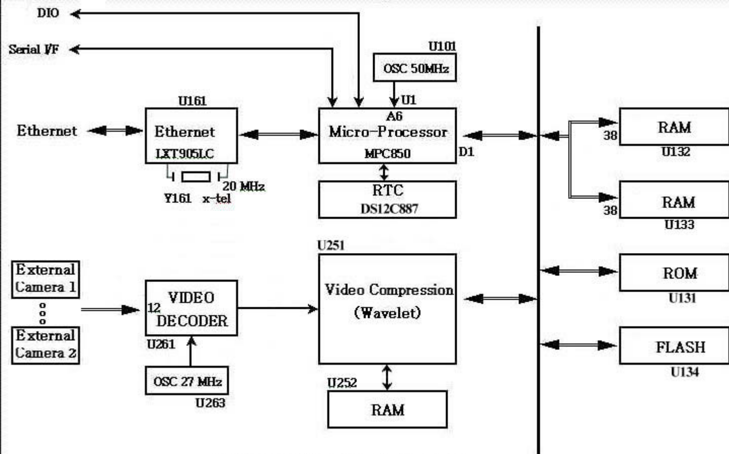
WebEye B101 Block Diagram
