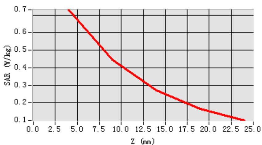
SAR, Z Axis Scan (X = -23, Y = -23)
