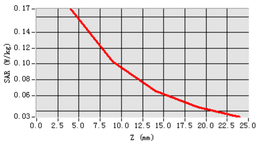
SAR, Z Axis Scan (X = -12, Y = -35)
