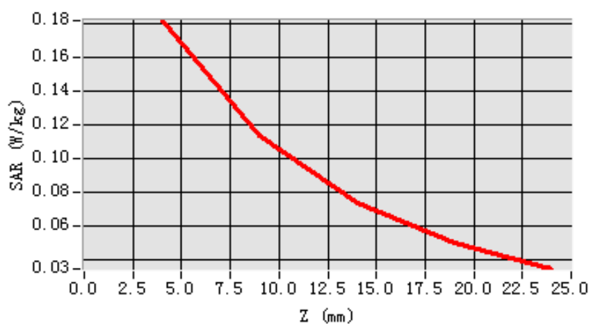
SAR, Z Axis Scan (X = 3, Y = 27)
