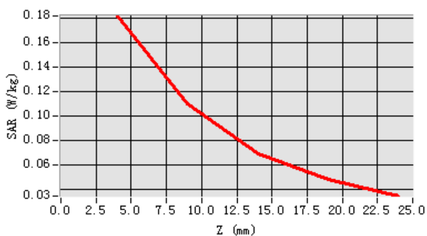
SAR, Z Axis Scan (X = -12, Y = -41)
