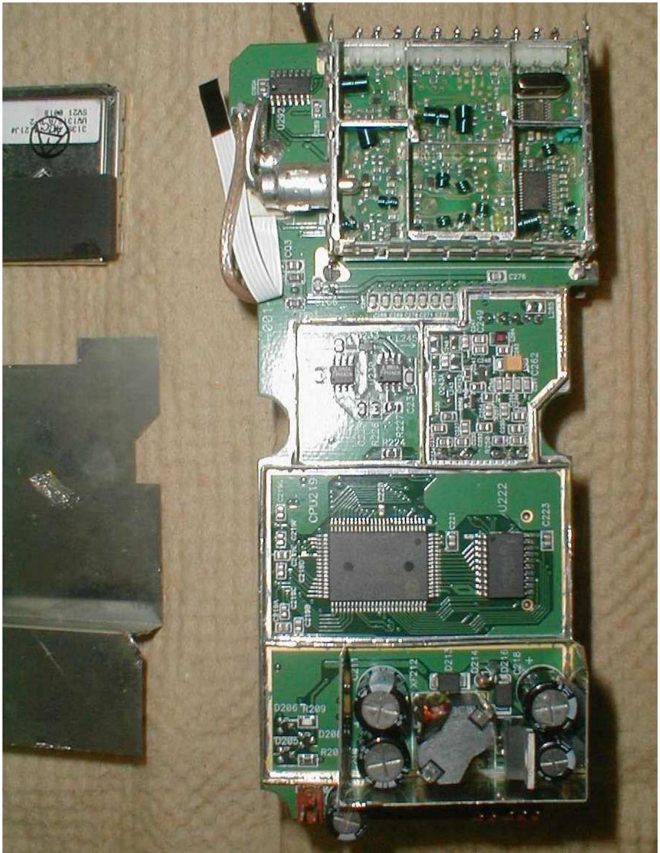
Shield 3 and Phillips Module Top Shield Removed
