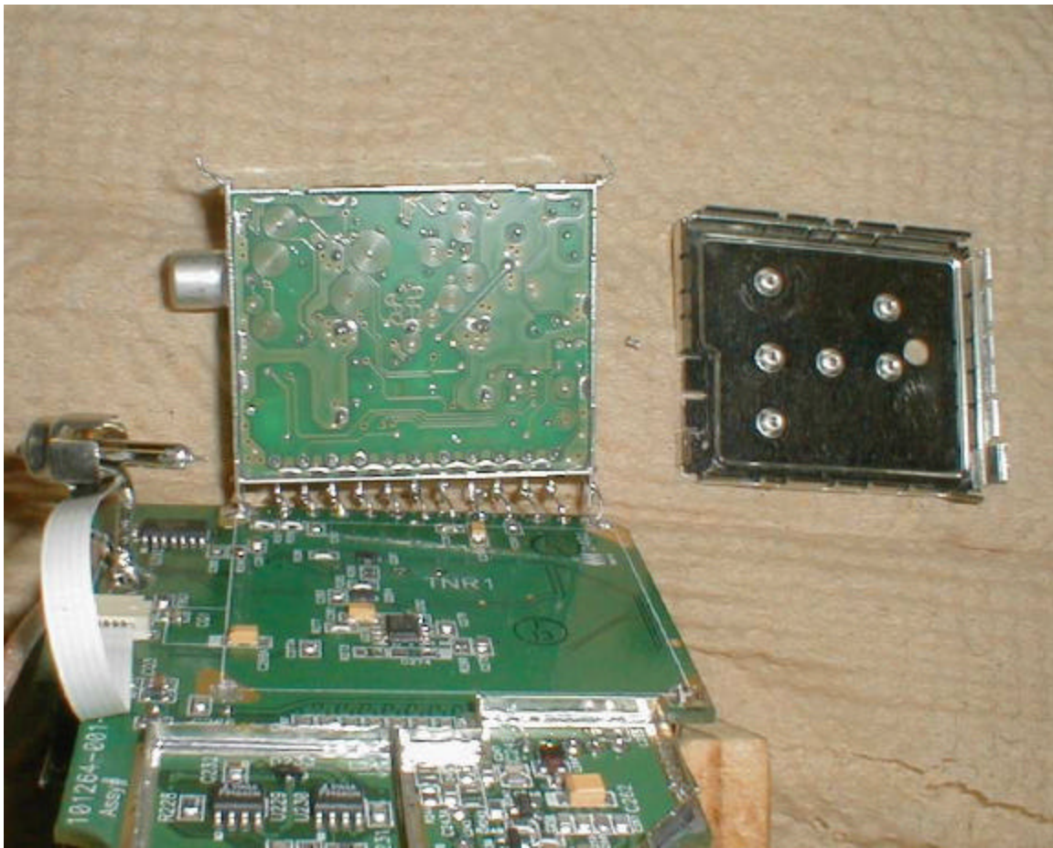
Phillips Module Bottom View, Shield Removed
