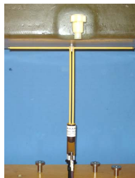
SPEAG 300 MHz Validation Dipole Setup
