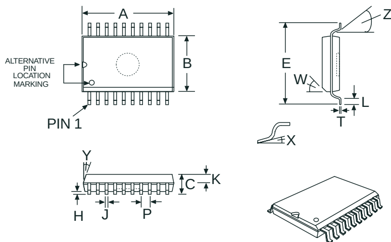
Figure 15: 20-pin SOIC Mechanical Outline: Order as part no. MX469D3
