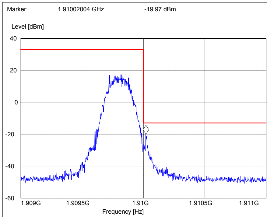
Picture 6 Upper bandedge, EGPRS 1900 channel 810, flip closed
