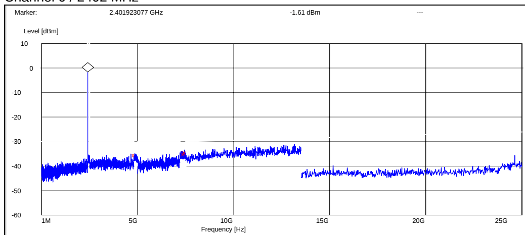
Channel 0 / 2402 MHz
