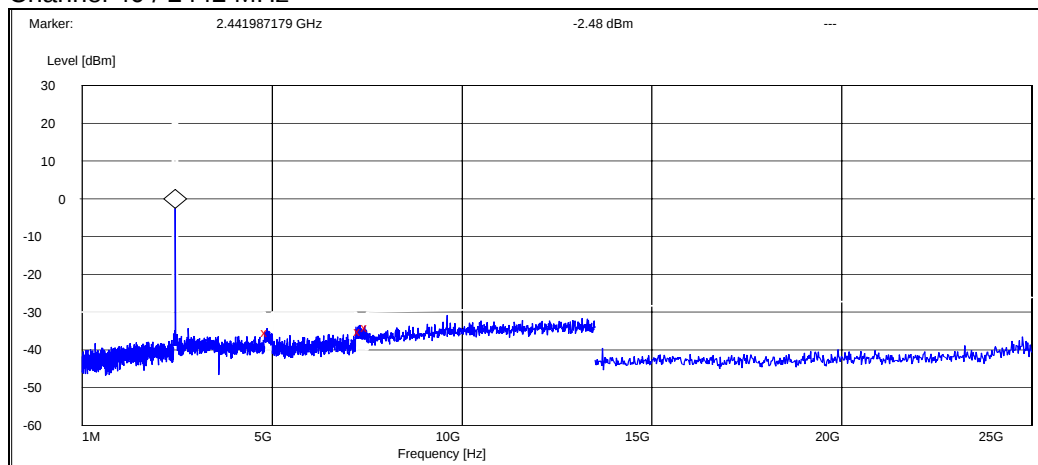
Channel 40 / 2442 MHz
